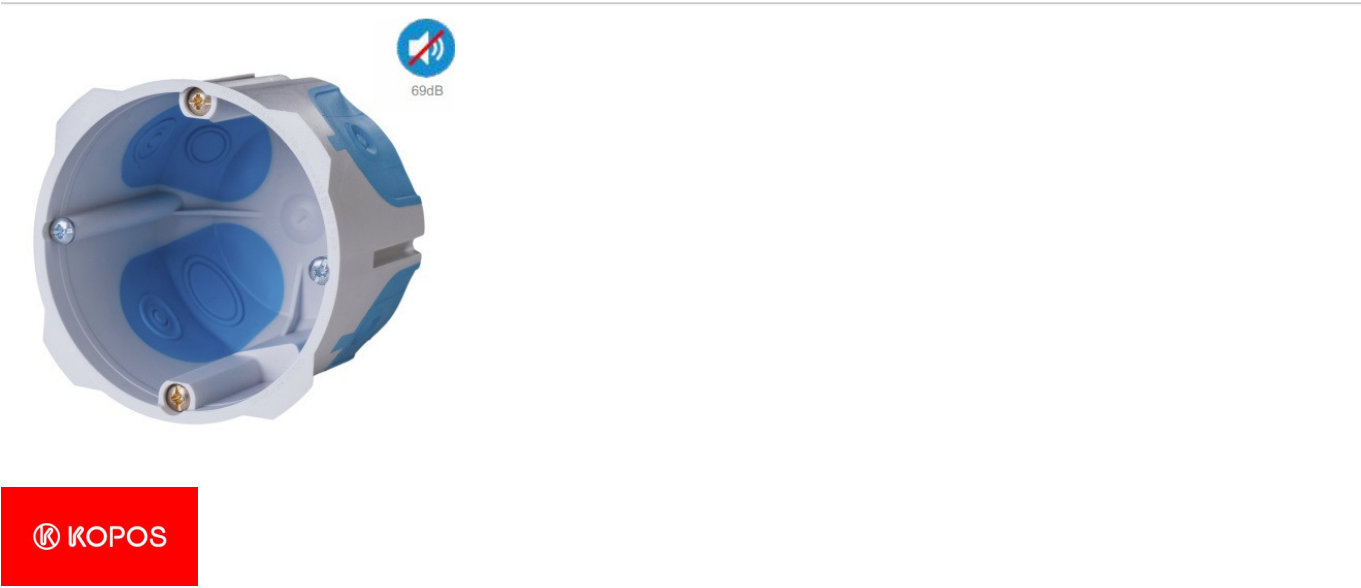
Windproof Cavity wall box with soft entries Hard version Halogen-free 1x60x68
