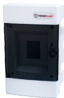
Enclosures Flush mounting - IP40 - 4 Modules235 x 139 x 98
